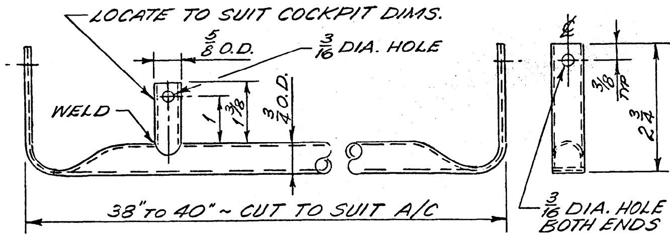
TORQUE ROD MAT'L: 5052-H32 ALUM. TUBING
